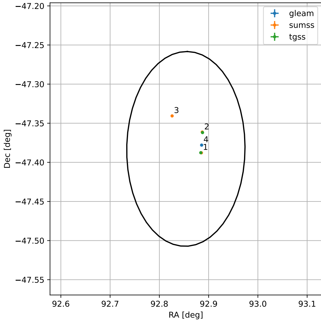
4FGL J0611.4-4722
