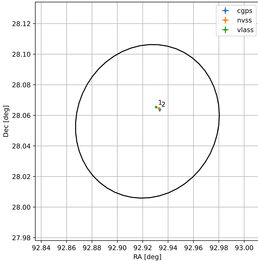
4FGL J0611.6+2803
