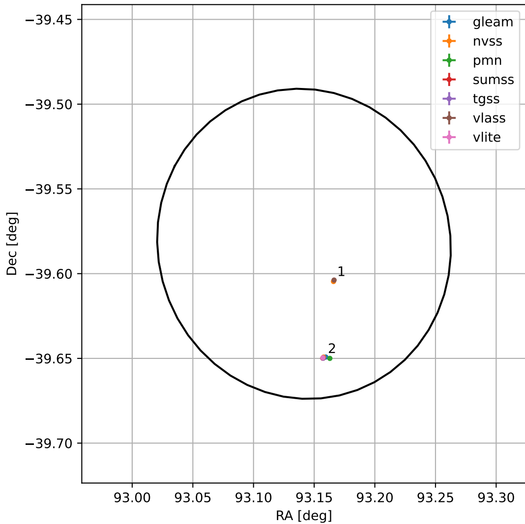
4FGL J0612.5-3934
