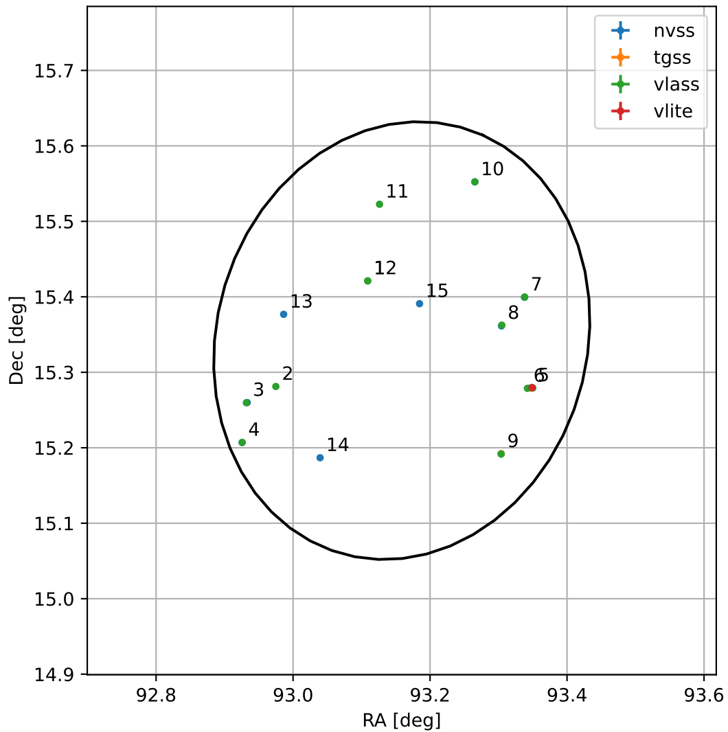
4FGL J0612.6+1520
