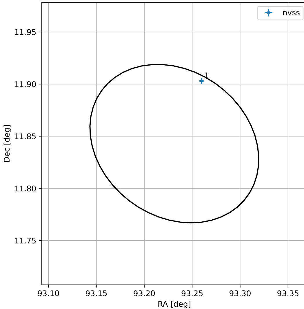
4FGL J0612.9+1150
