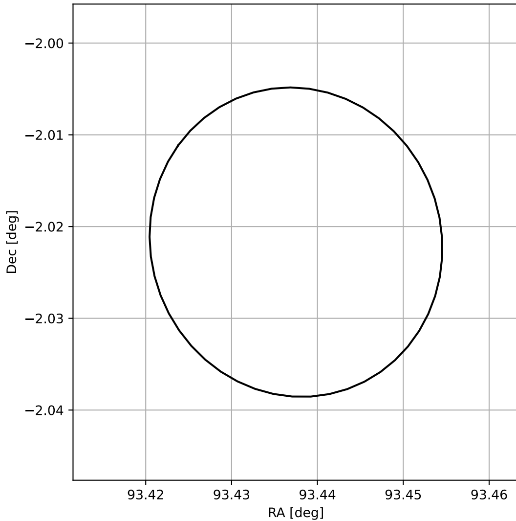
4FGL J0613.7-0201
