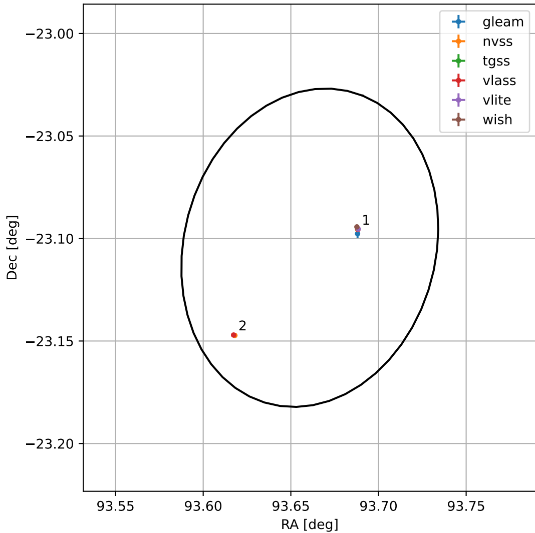
4FGL J0614.6-2306
