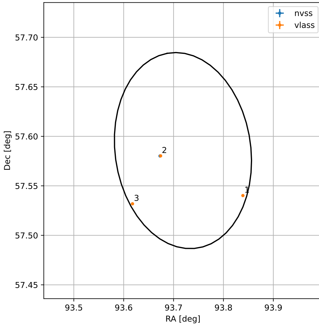
4FGL J0614.8+5735
