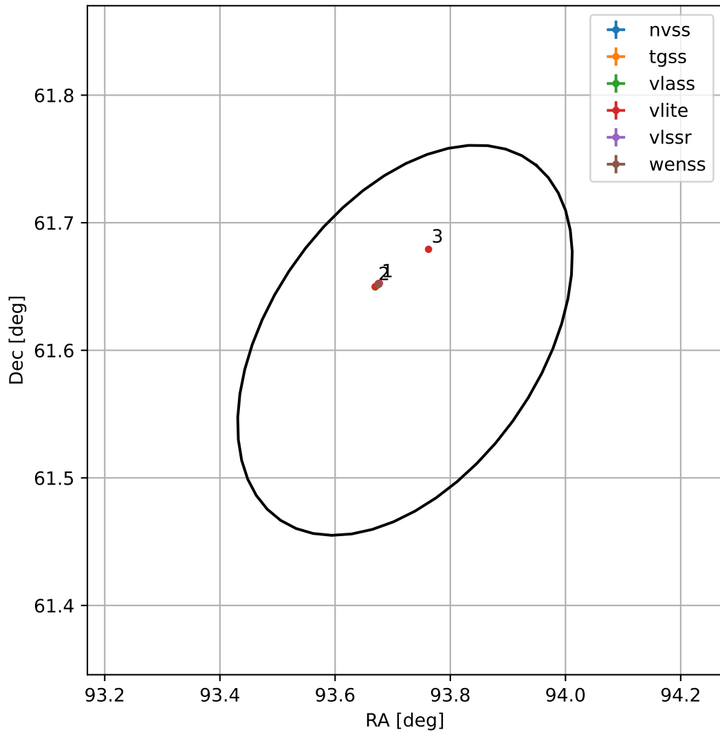
4FGL J0614.8+6136
