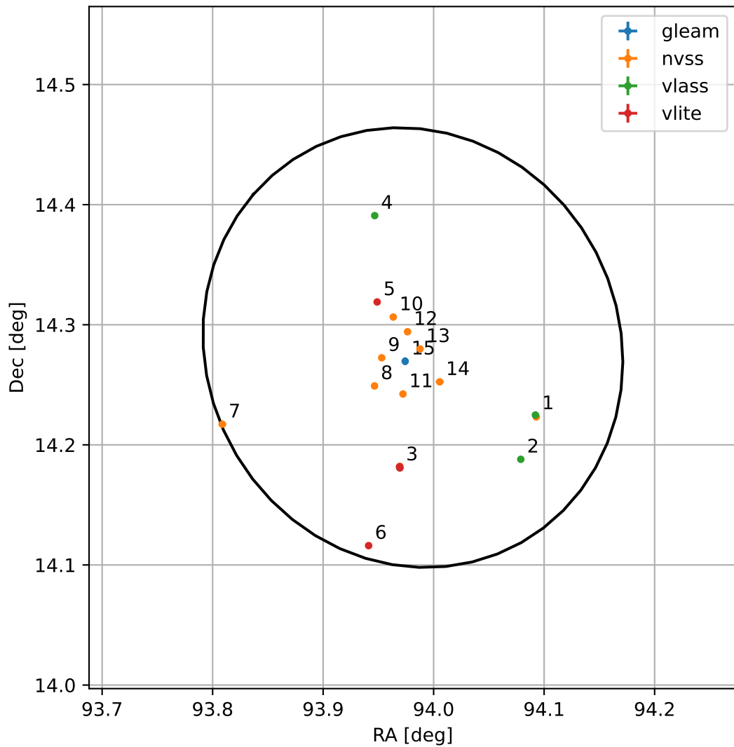
4FGL J0615.9+1416
