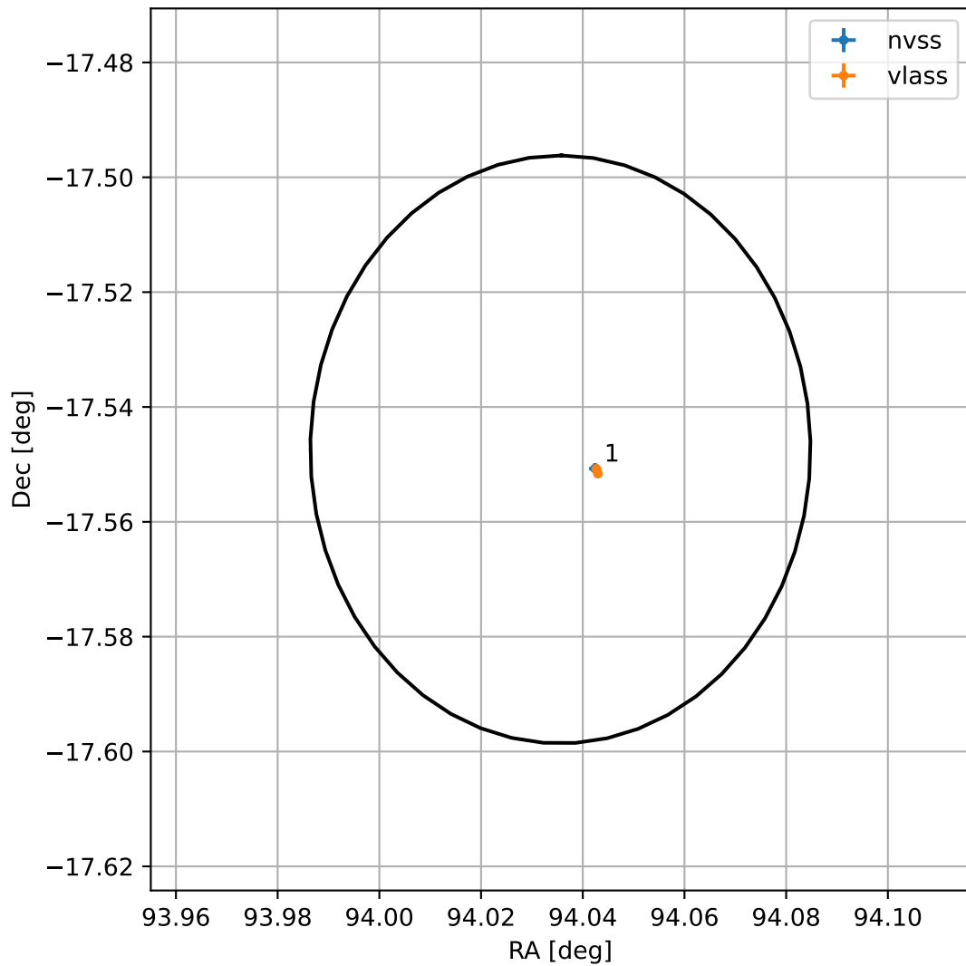
4FGL J0616.1-1732
