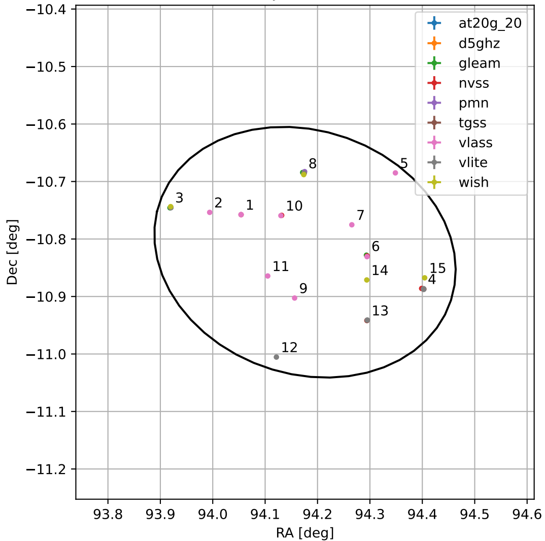
4FGL J0616.7-1049
