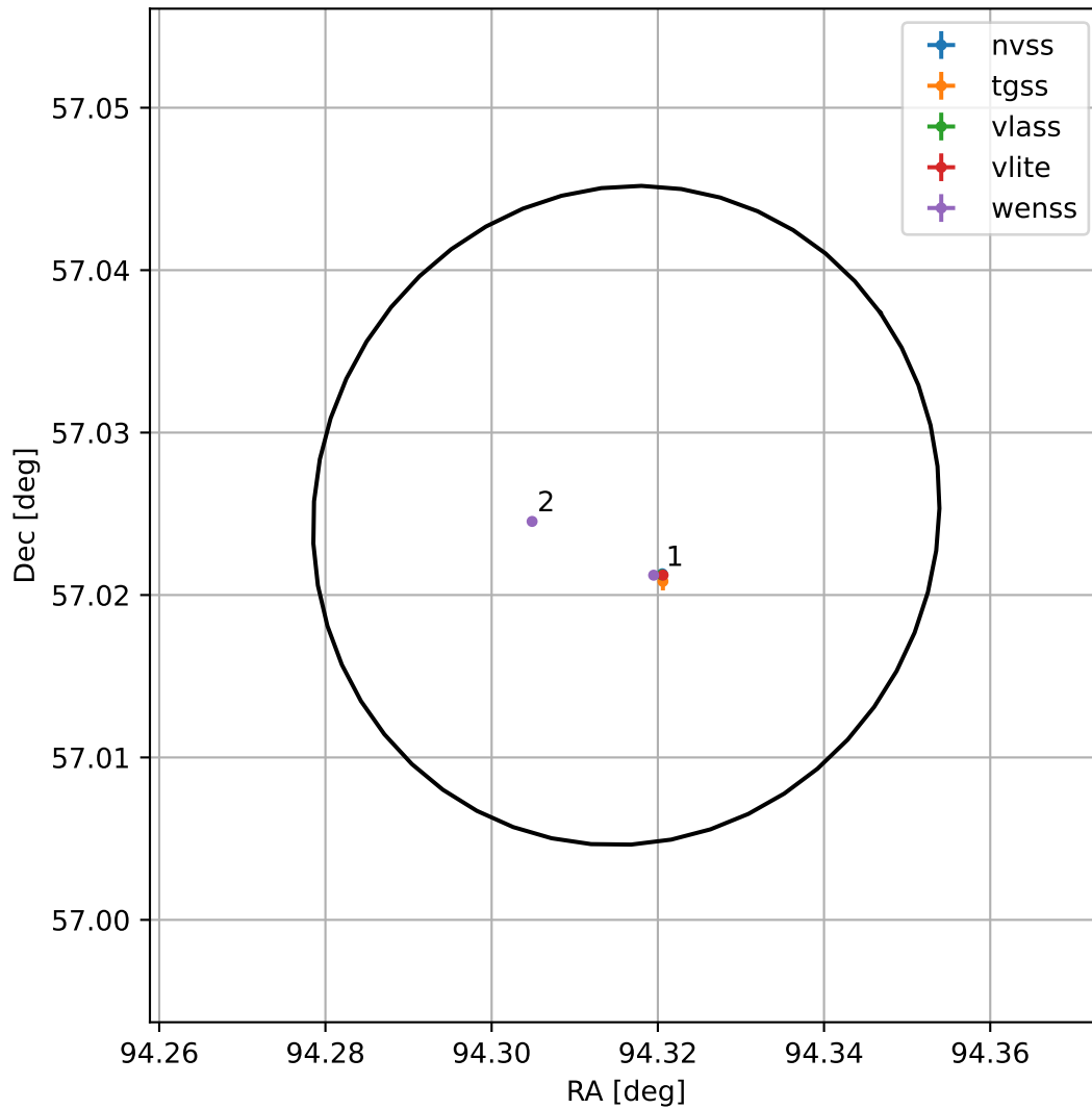
4FGL J0617.2+5701
