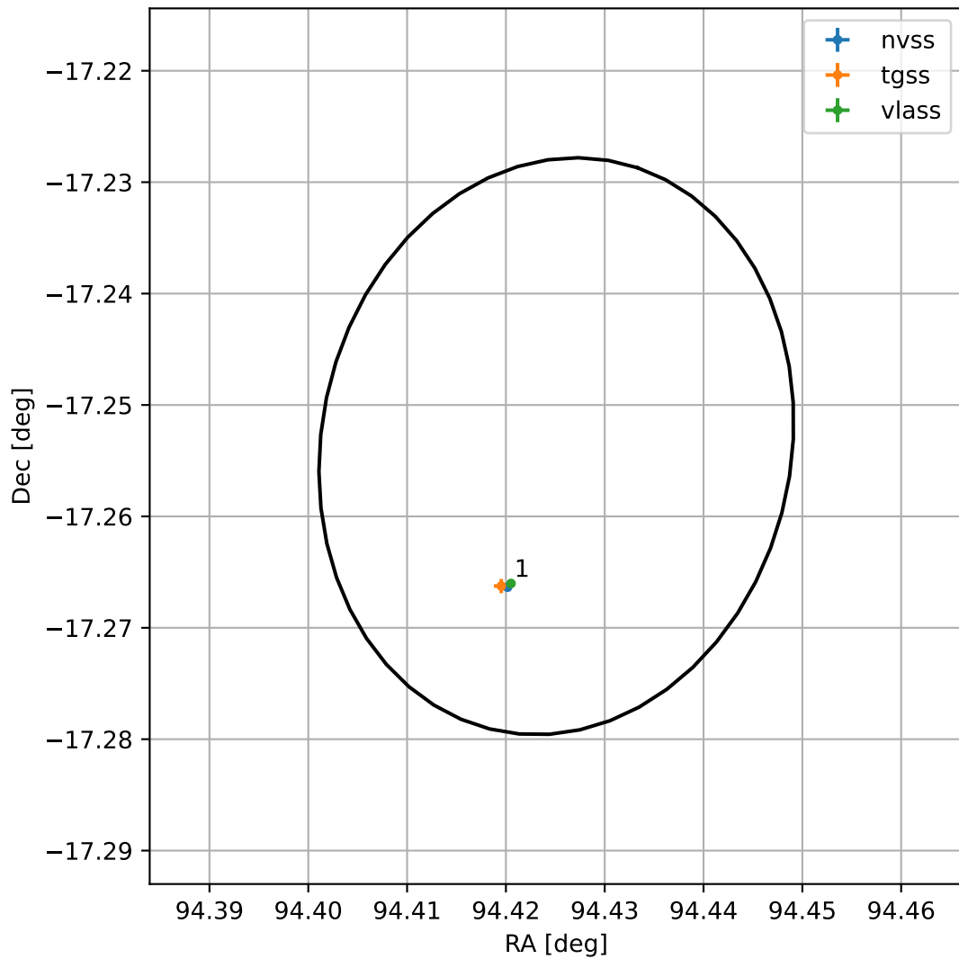
4FGL J0617.7-1715
