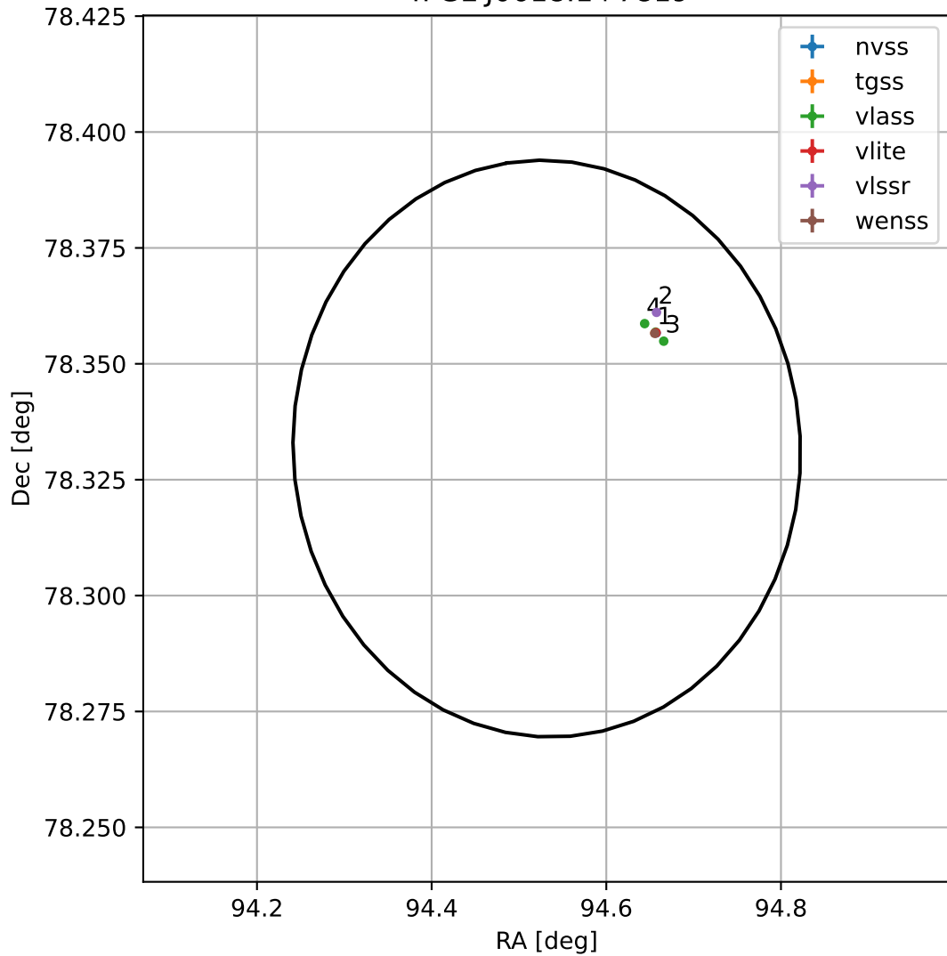
4FGL J0618.1+7819
