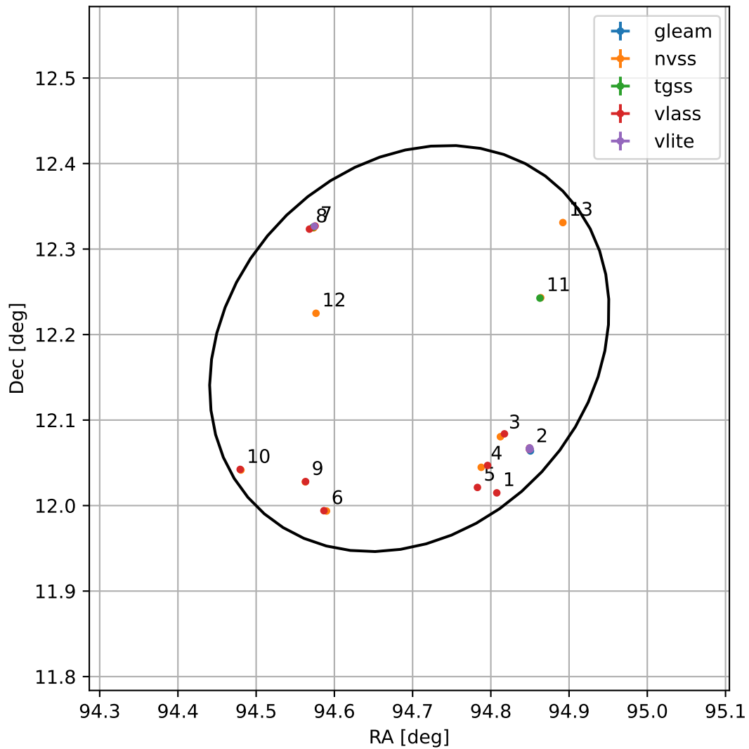
4FGL J0618.7+1211
