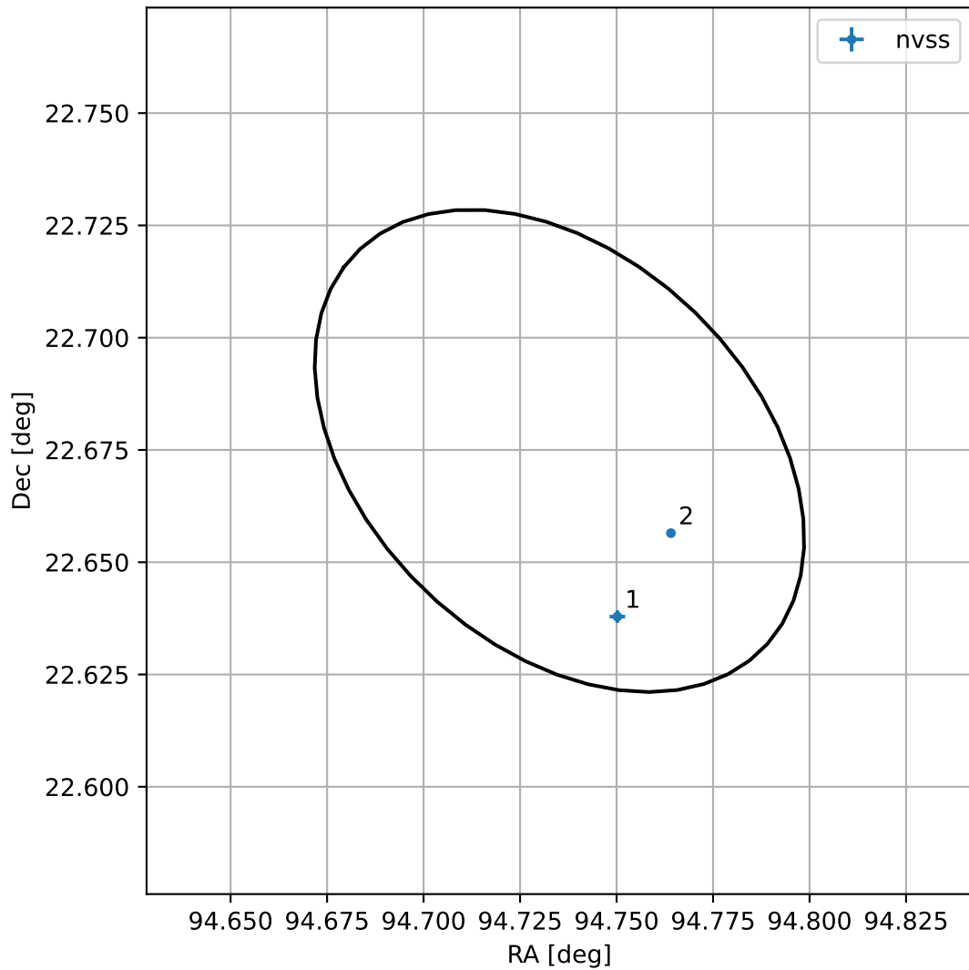
4FGL J0618.9+2240
