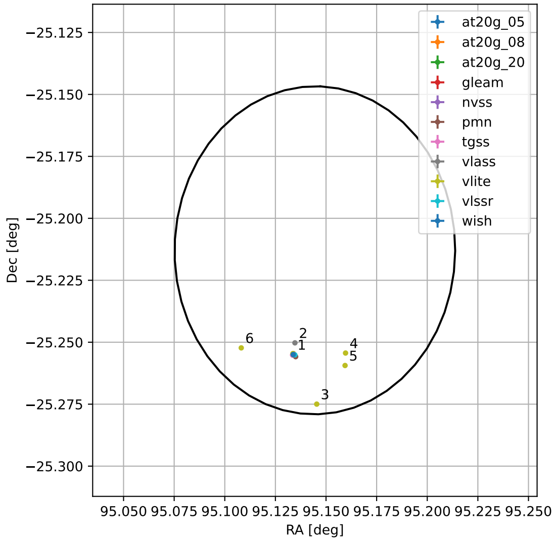
4FGL J0620.5-2512
