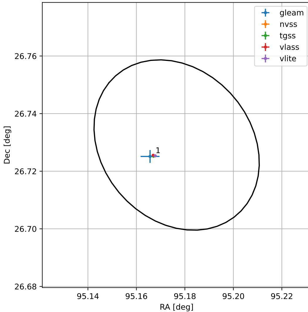
4FGL J0620.7+2643
