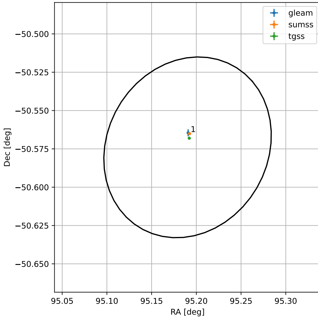
4FGL J0620.7-5034
