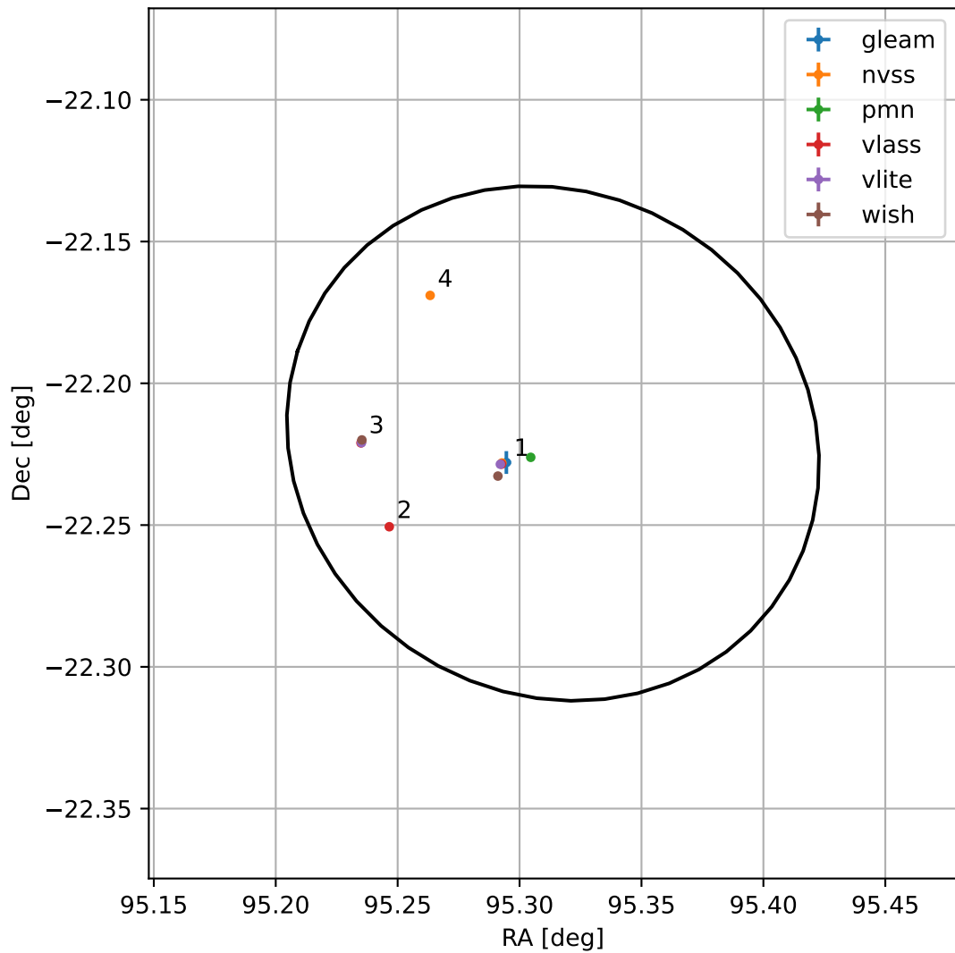
4FGL J0621.2-2213
