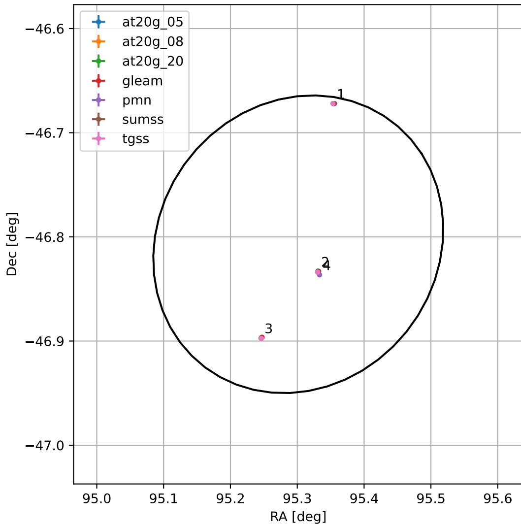
4FGL J0621.2-4648
