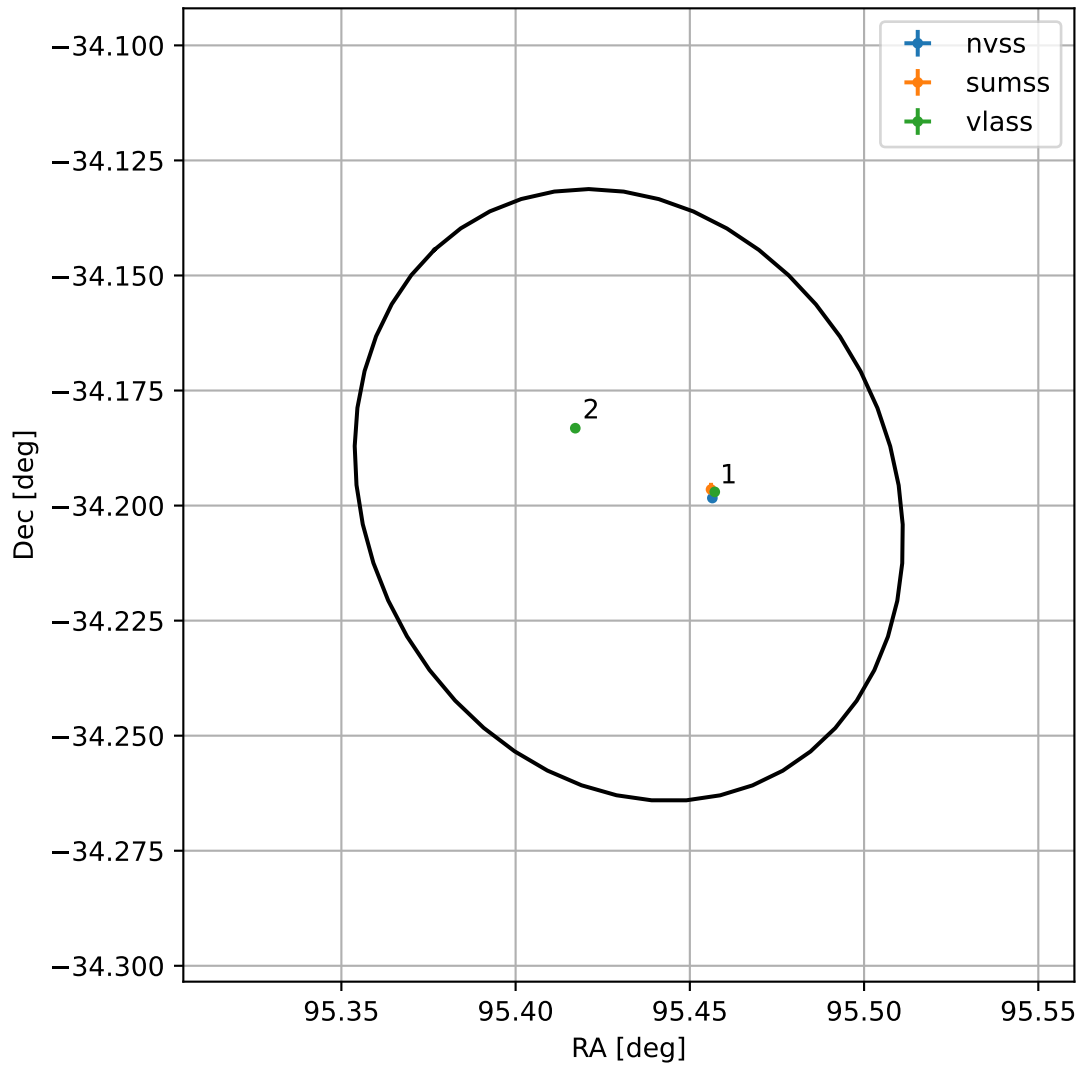
4FGL J0621.7-3411
