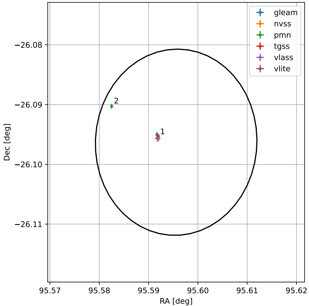
4FGL J0622.3-2605
