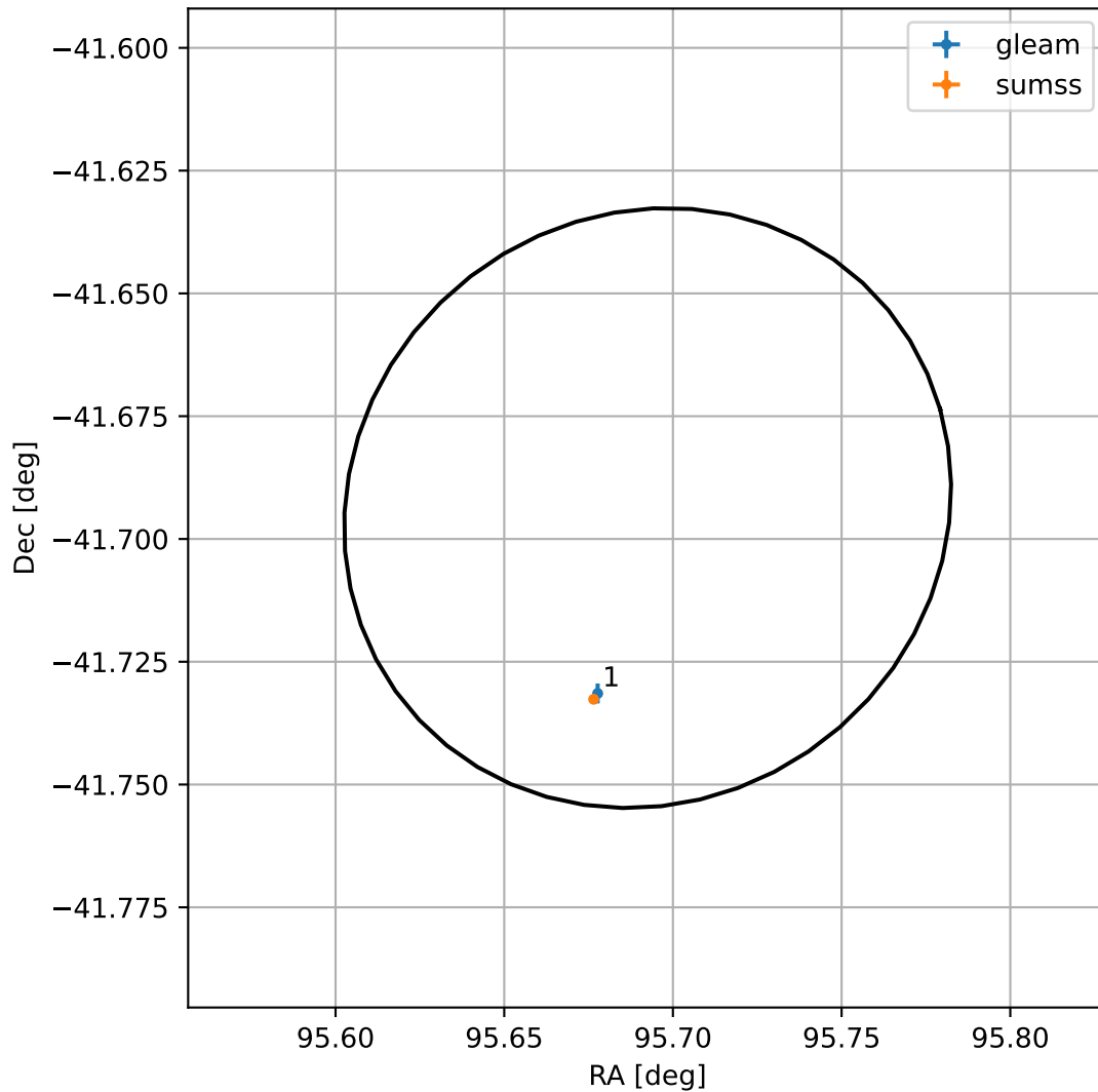
4FGL J0622.7-4141
