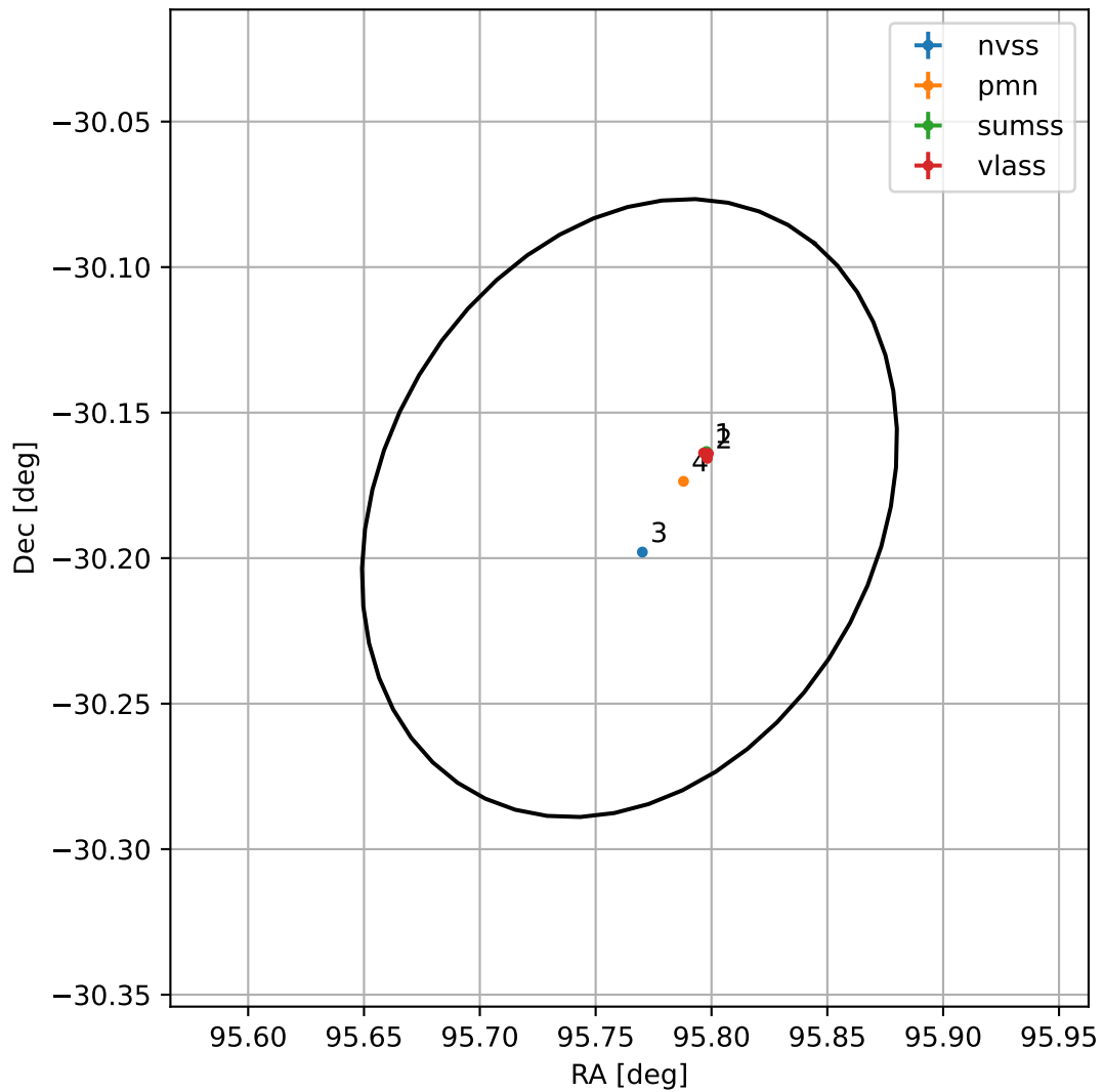
4FGL J0623.0-3010
