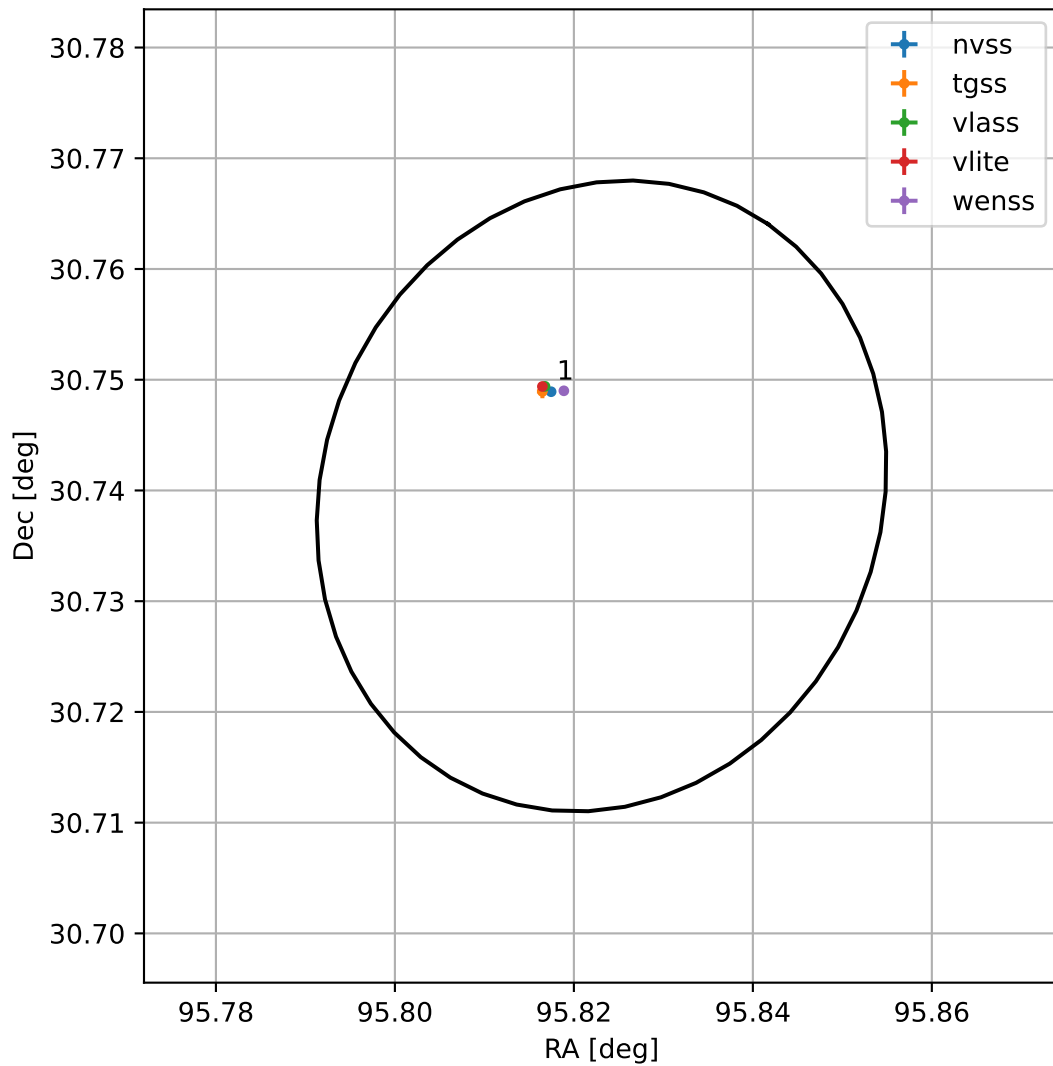
4FGL J0623.2+3044
