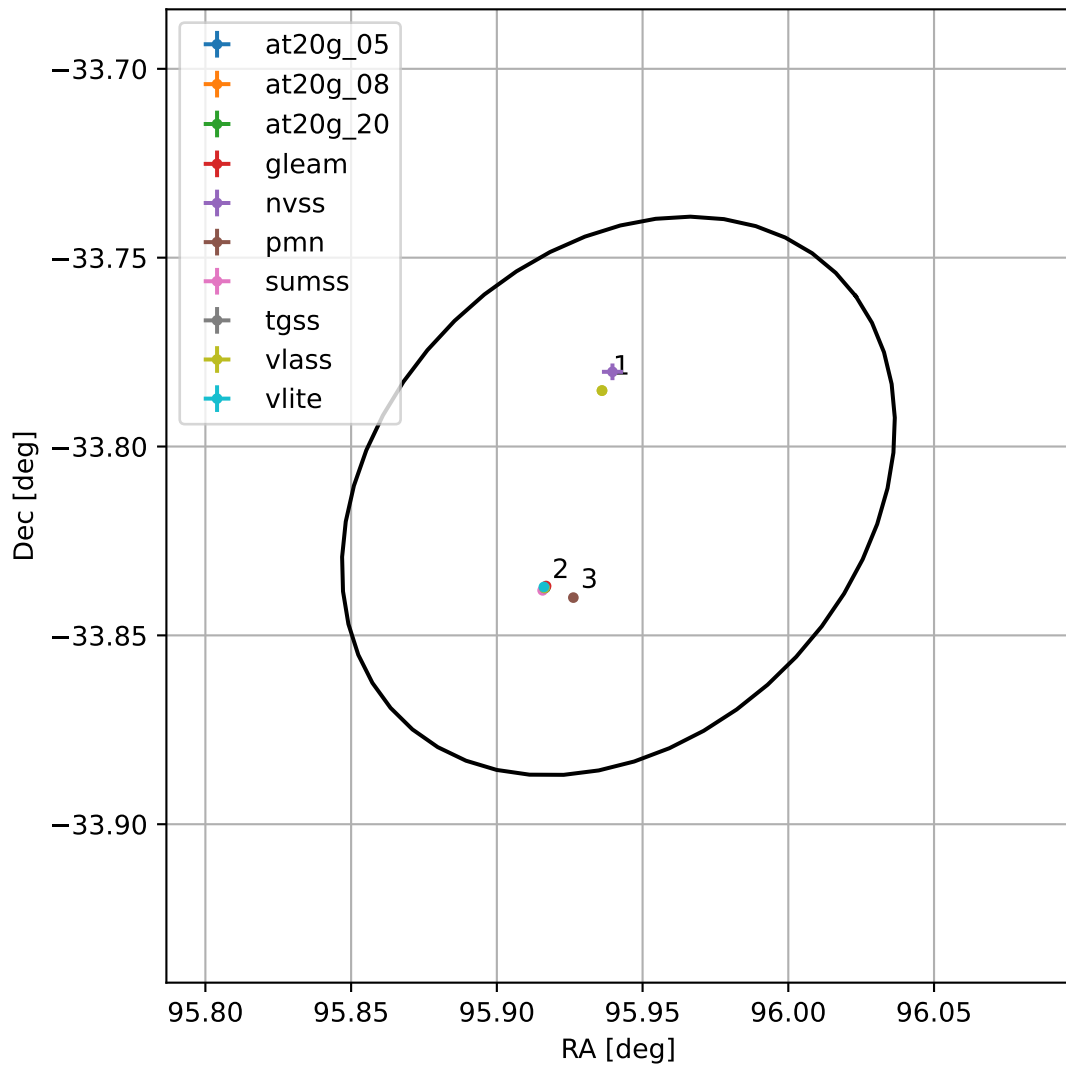
4FGL J0623.7-3348
