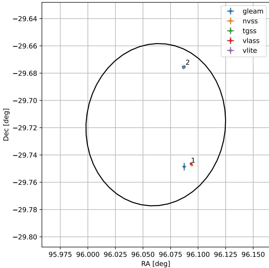
4FGL J0624.2-2943
