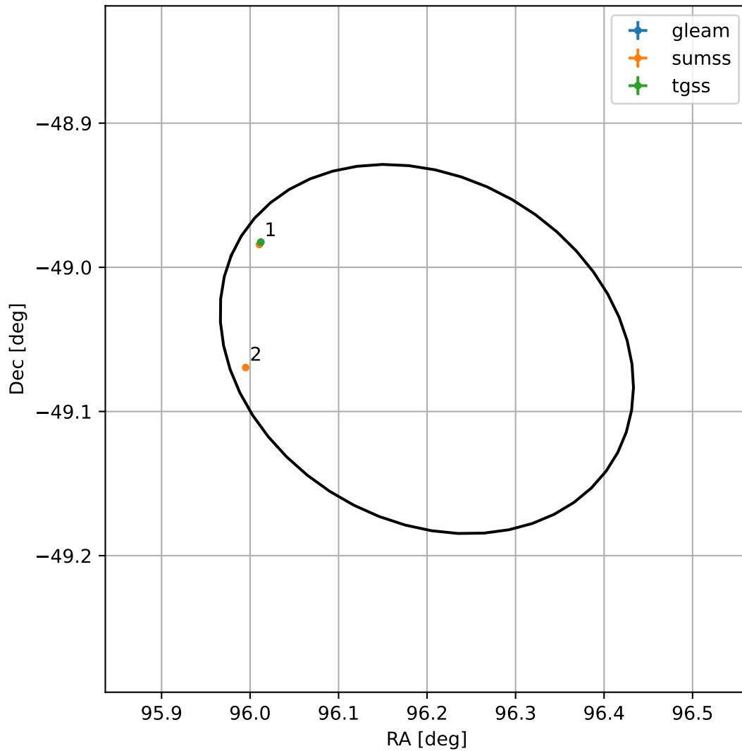
4FGL J0624.7-4903
