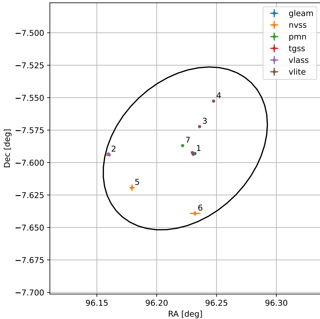
4FGL J0624.8-0735
