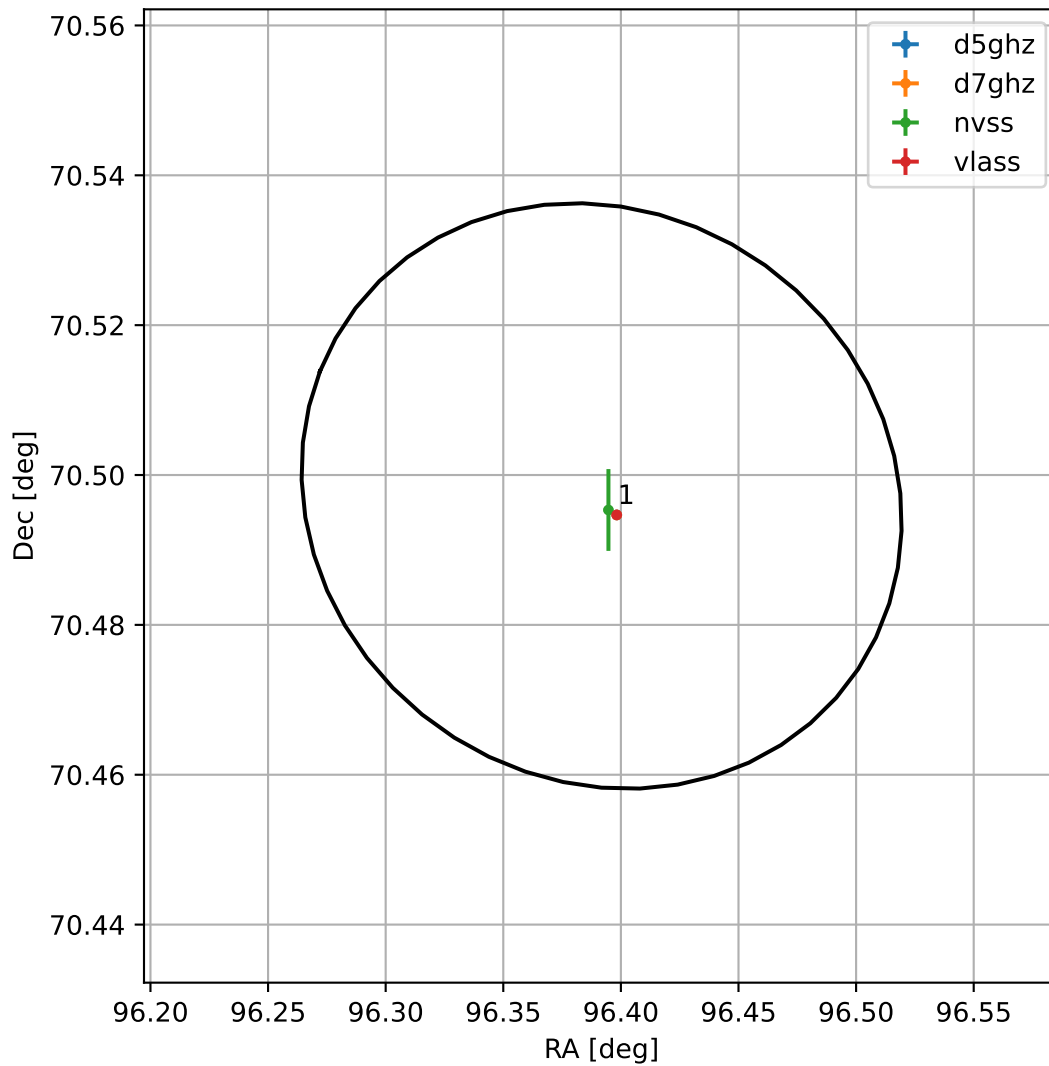
4FGL J0625.5+7029
