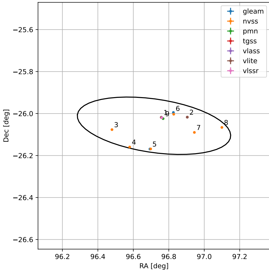
4FGL J0626.8-2603
