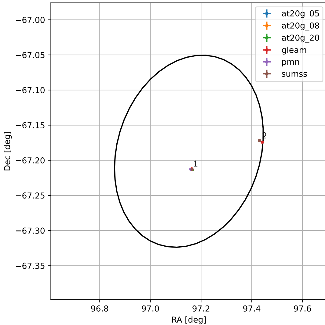
4FGL J0628.6-6711
