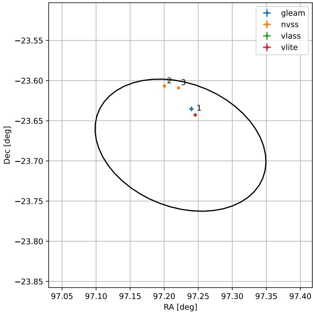
4FGL J0628.8-2340
