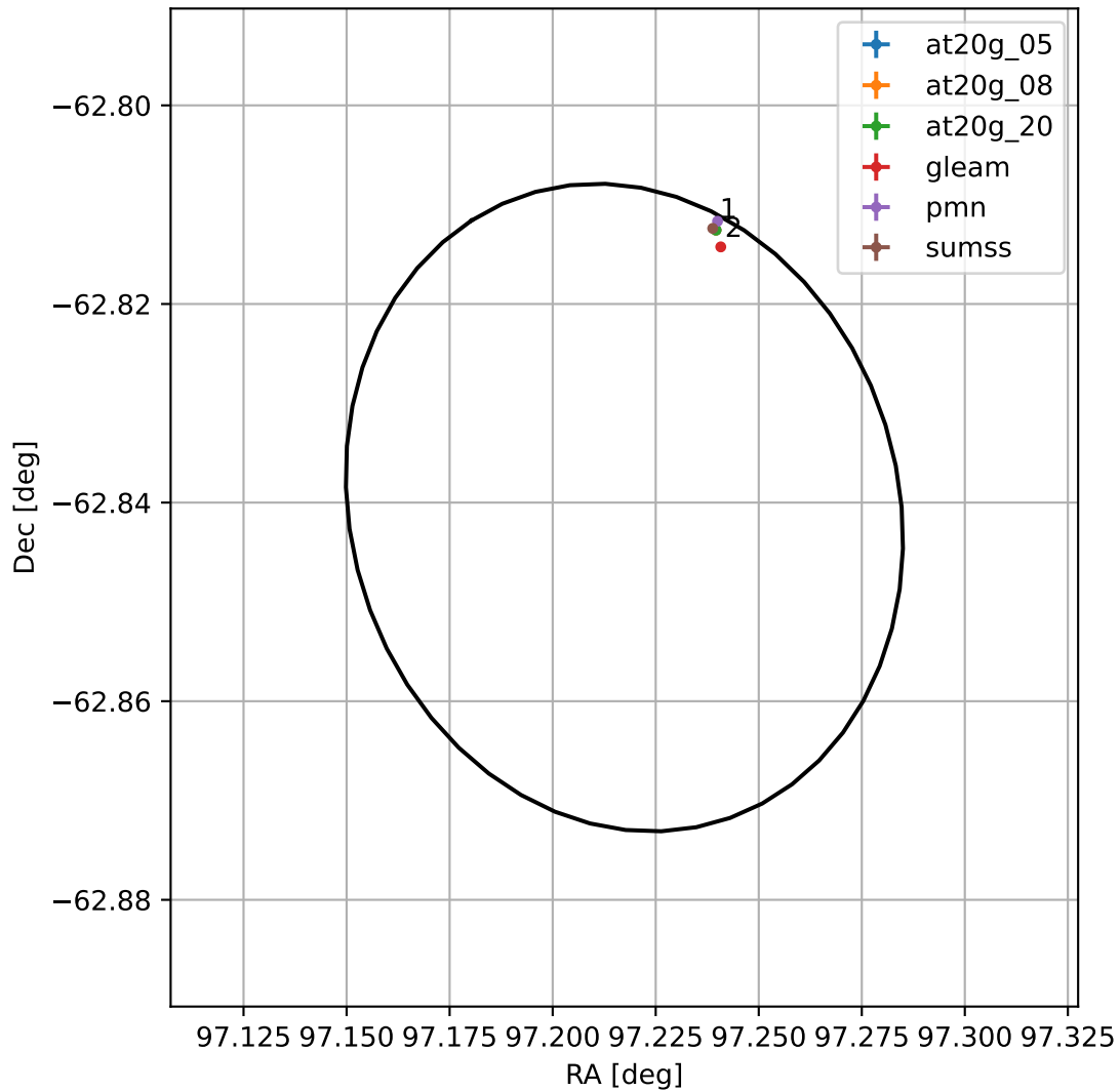
4FGL J0628.8-6250
