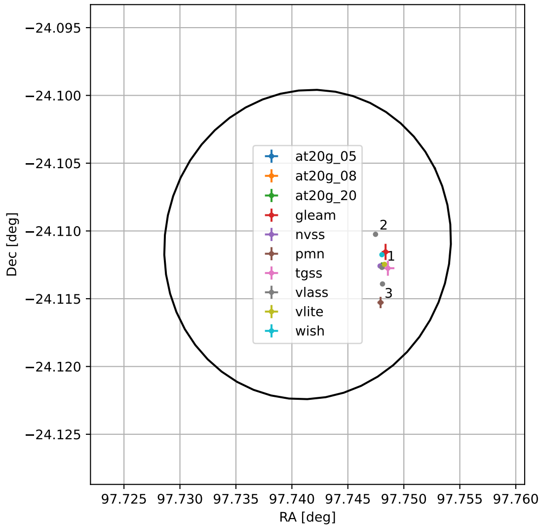
4FGL J0630.9-2406
