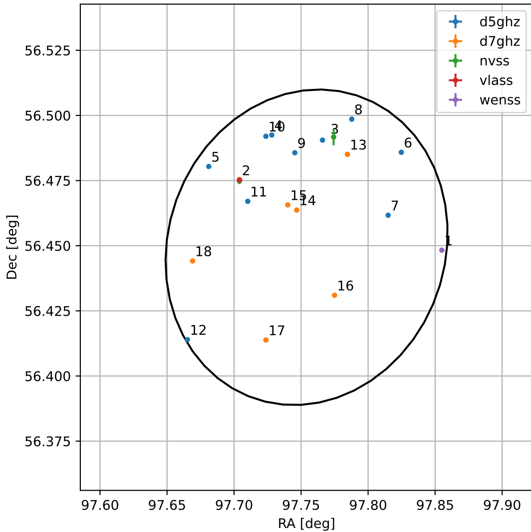
4FGL J0631.0+5626
