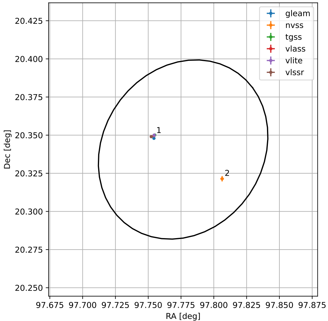
4FGL J0631.1+2020
