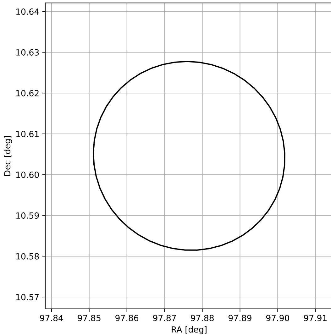
4FGL J0631.5+1036
