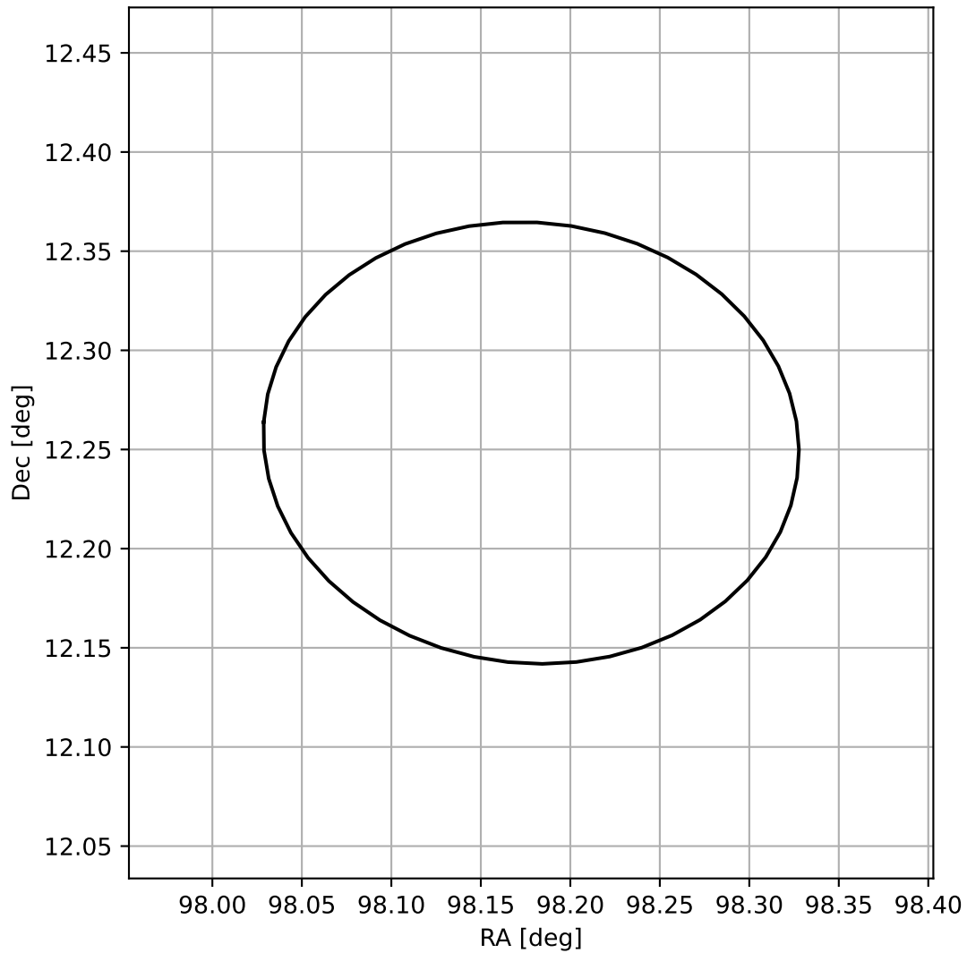
4FGL J0632.7+1215
