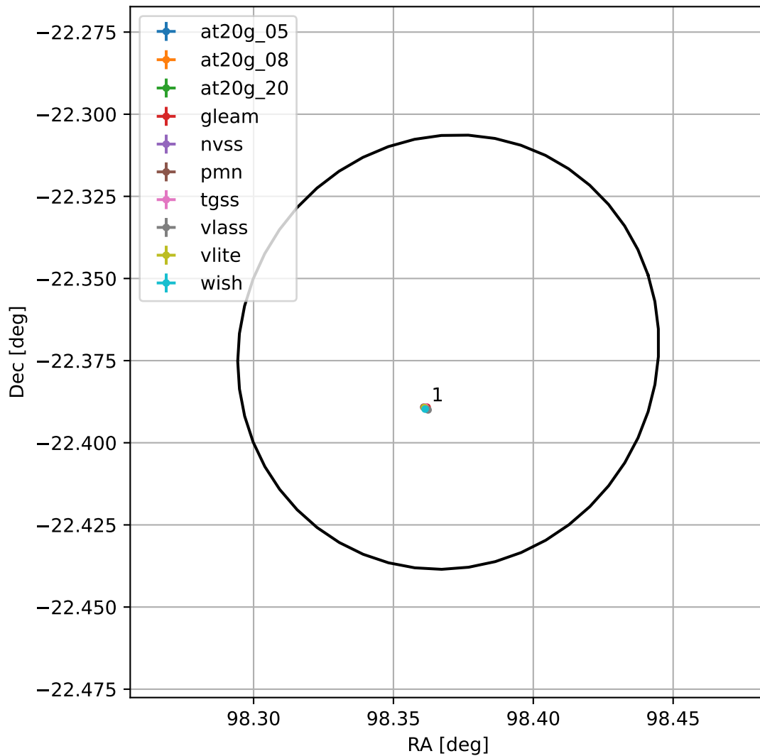
4FGL J0633.4-2222
