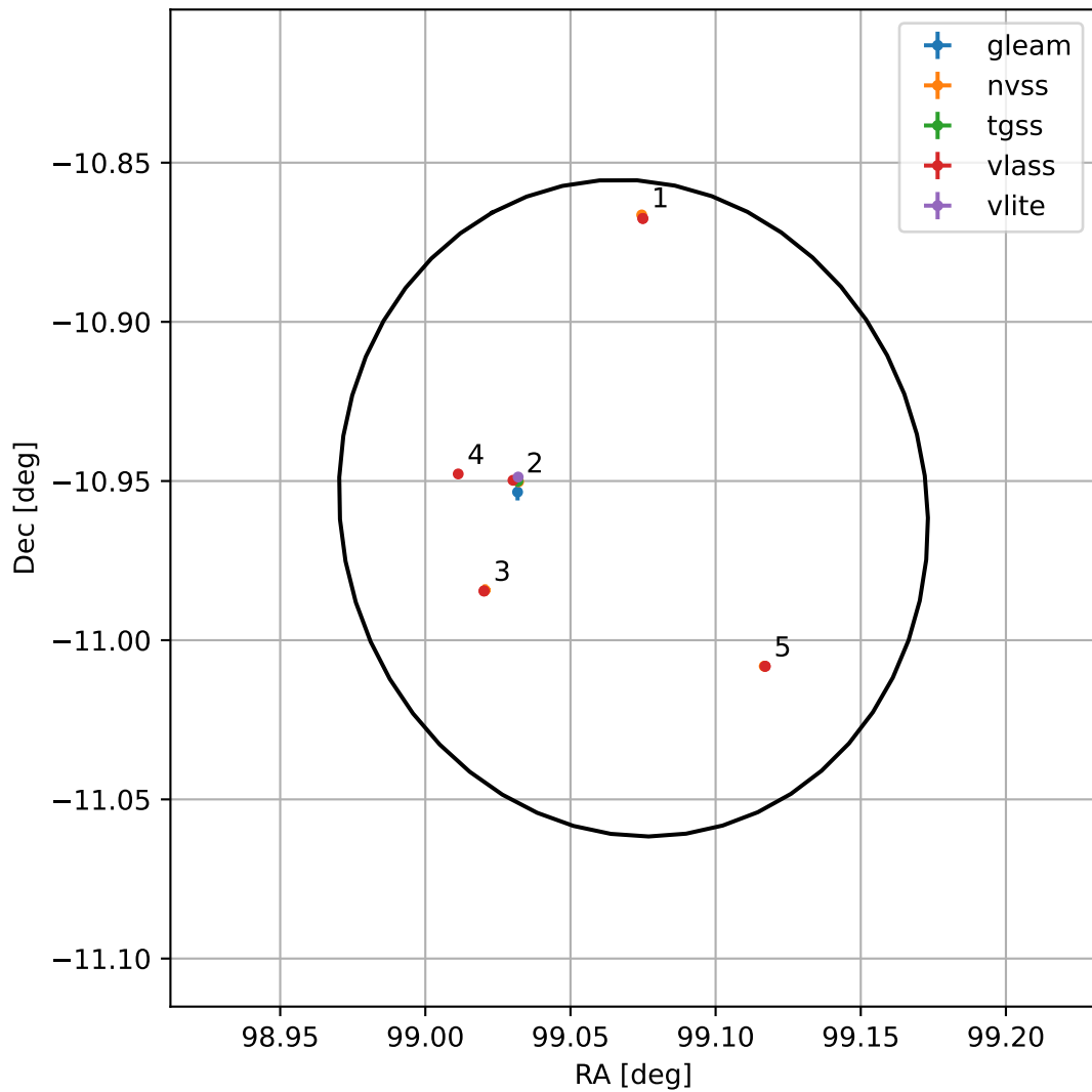
4FGL J0636.2-1057
