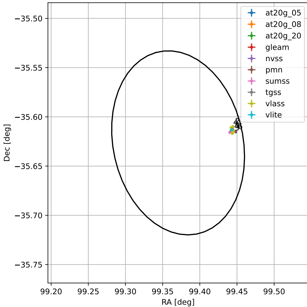
4FGL J0637.4-3537
