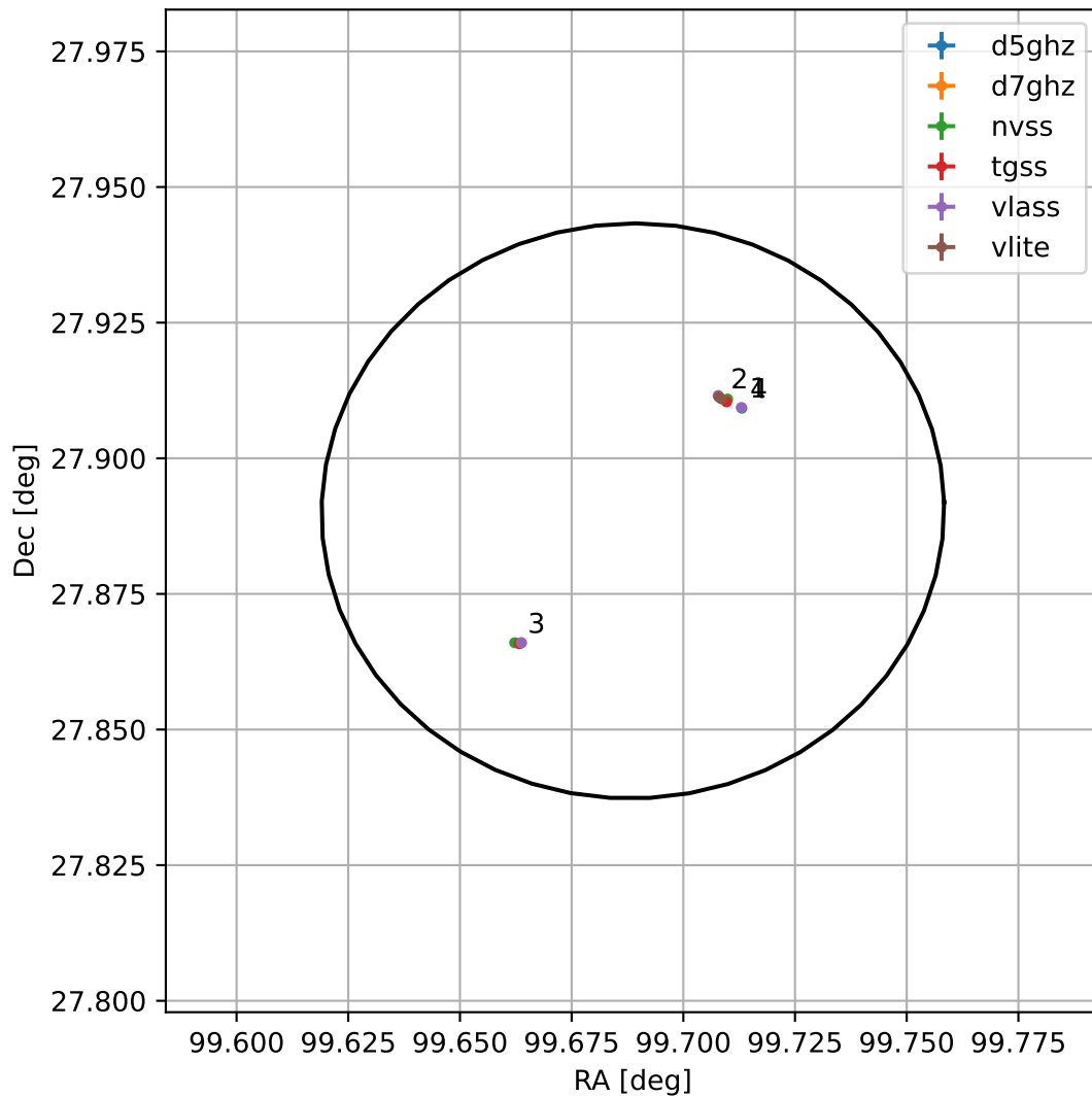
4FGL J0638.7+2753
