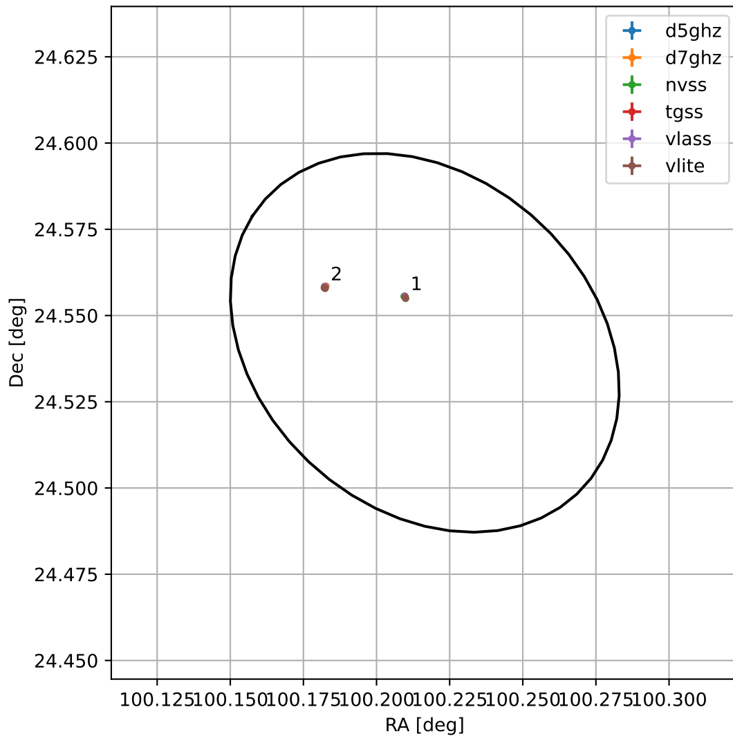
4FGL J0640.8+2432
