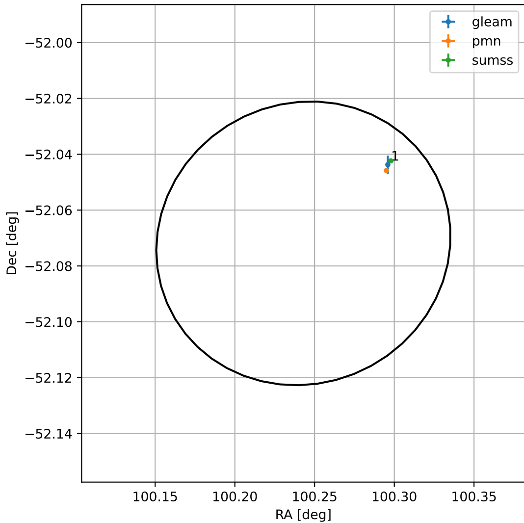
4FGL J0640.9-5204
