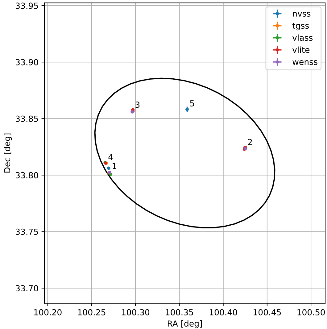
4FGL J0641.4+3349
