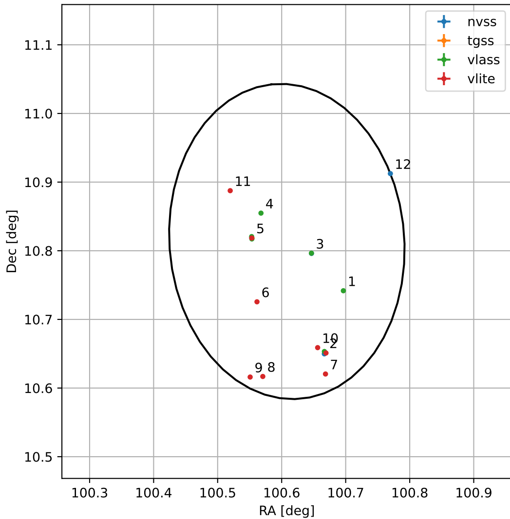
4FGL J0642.4+1048
