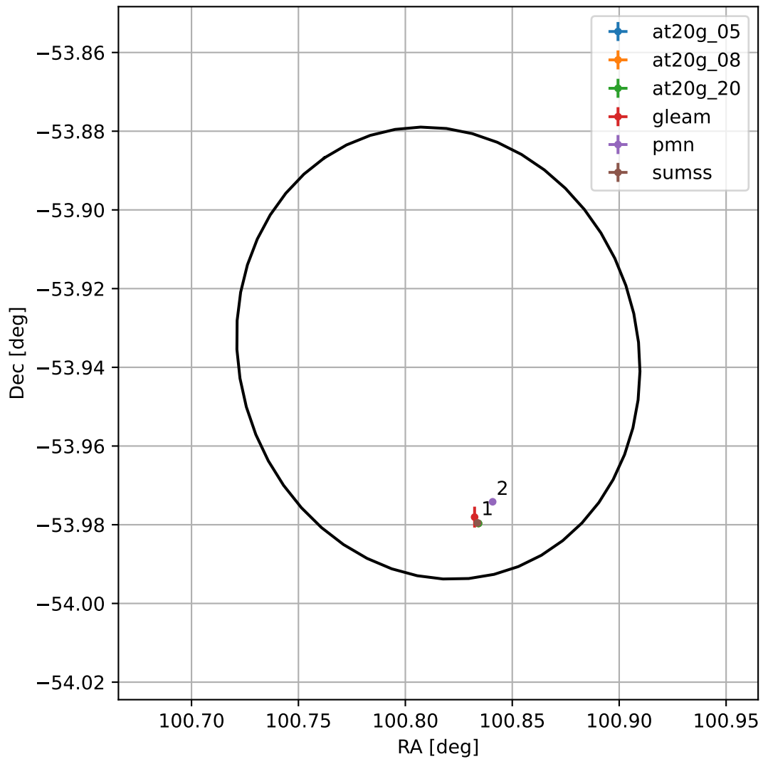
4FGL J0643.2-5356
